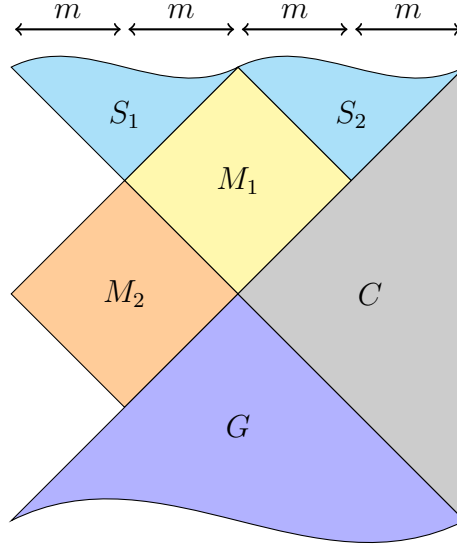
FIGURE 14. Construction for Theorem 2: splitters S_1, S_2 , matrix gadgets M_1, M_2 , merger G , and a tangle C from Proposition 15.
