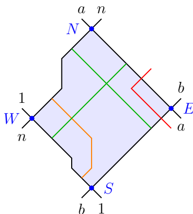
FIGURE 18. Illustration of the proof of Lemma 19: the region formed by paths a, b, 1, n , and the four types of path that may intersect it. An RL path necessitates an LR path, but an LR path requires two further moves in order to cross paths n and 1 .
