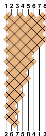
(b) A greedy construction of such a tangle: we apply alternate rows of swaps in odd and even positions until path \pi(n) is in the rightmost position, then continue in the same way with locations 1, \dots, n - 1 .
