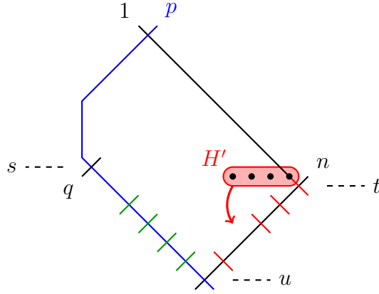
FIGURE 17. The key step in the proof of Proposition 5. The paths of H' must all cross path n before time s , therefore at least as many paths must cross path p during the same time interval.
