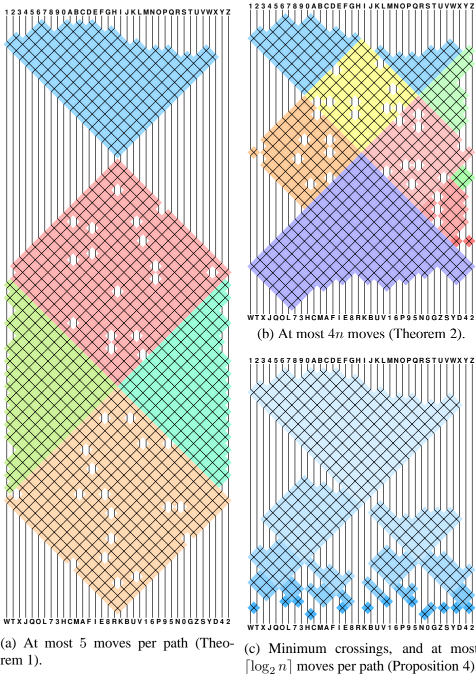
FIGURE 2. Examples of the tangles corresponding to the main results. Shading is added to illustrate the structure.
