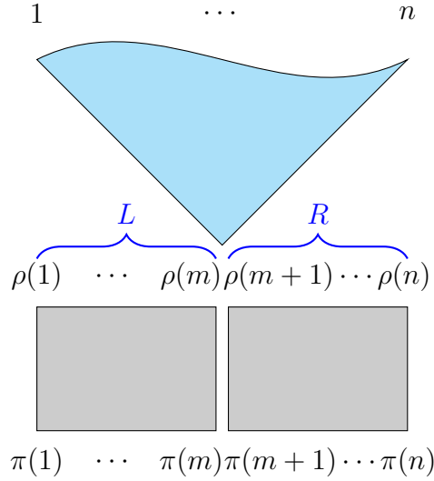
FIGURE 10. Construction for Proposition 4. After the initial splitter, the two rectangles signify smaller recursively defined versions of the same construction.
