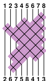
(a) A tangle occupying a simply connected region bounded by monotone interfaces, as discussed in open problem 4.
