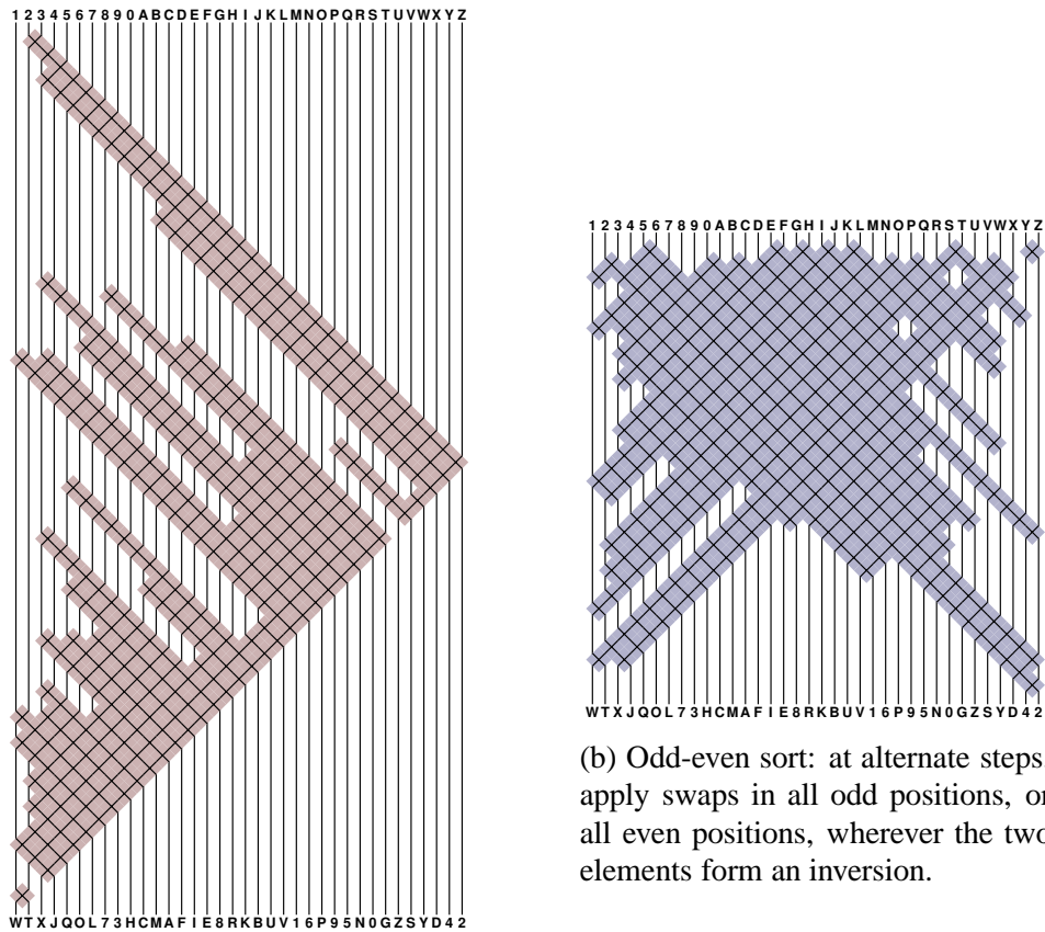
(a) Bubble sort variant: use one R-move to route each path to its correct position, starting from the rightmost, \pi(n) . Path i may have \Omega(i) L-moves.
