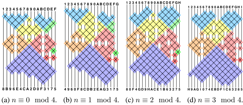
FIGURE 15. Variations of the construction for Theorem 2, according to the congruence class of n .
