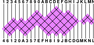
FIGURE 5. A direct tangle, performing a 321-avoiding permutation.
