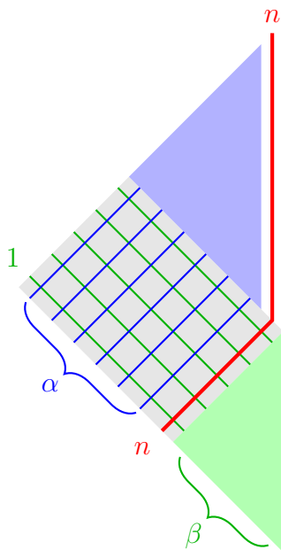
FIGURE 9. Inductive construction of a right reflector. The rectangle is chosen so as to route path n to its correct location, and the two remaining triangles are then filled with smaller right reflectors.
