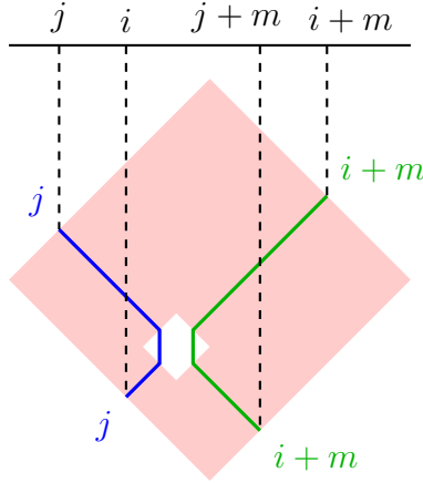
FIGURE 7. A pair of complementary paths in a matrix gadget. Horizontal positions are indicated along the top line.
