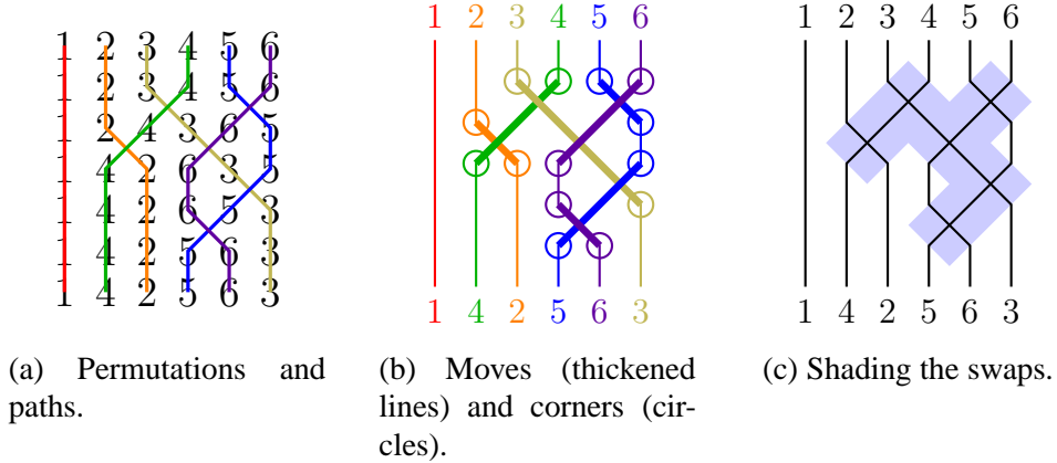
FIGURE 1. A tangle performing the permutation \pi = [1, 4, 2, 5, 6, 3] , with 7 moves.
