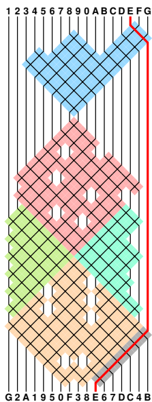
FIGURE 12. The construction for Theorem 1 for odd n : the largest element in the right half of the permutation is routed along the right side.
