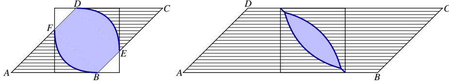
Figure 9: The measure \kappa_s : a point is picked uniformly in the parallelogram ABCD . If it is outside the curved polygon BEDF where \kappa_s is supported then it is shifted horizontally into the support. A similar description applies also for s > 1 .
