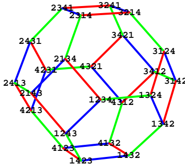
Figure 5: The permutahedron for n = 4 .
