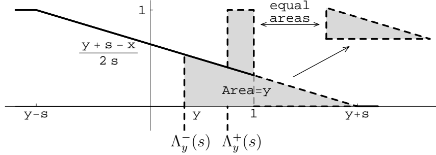
Figure 7: The functions \Lambda_y^-(s), \Lambda_y^+(s) .
