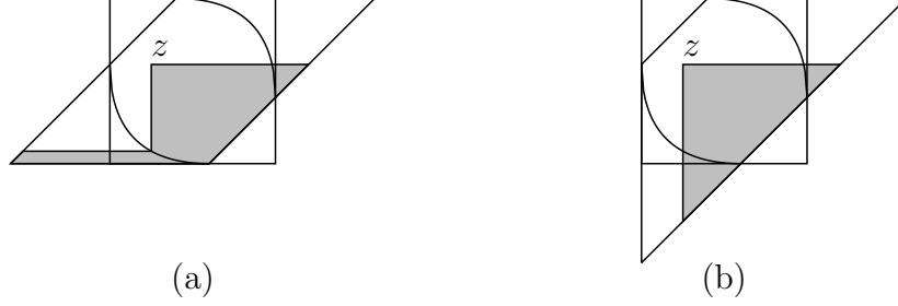
Figure 10: Proof of the claim when s \leq 1 : We will have z' \searrow z if the point from which z' is obtained by shifting the x -coordinate lies in the shaded region in (a). Symmetry of \kappa_s implies that the areas of the shaded regions in (a) and (b) are equal.
