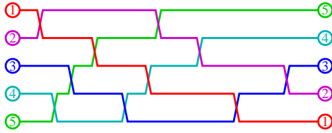
Figure 1: An illustration of an oriented swap process with n = 5 . Trajectories are shown by lines.
