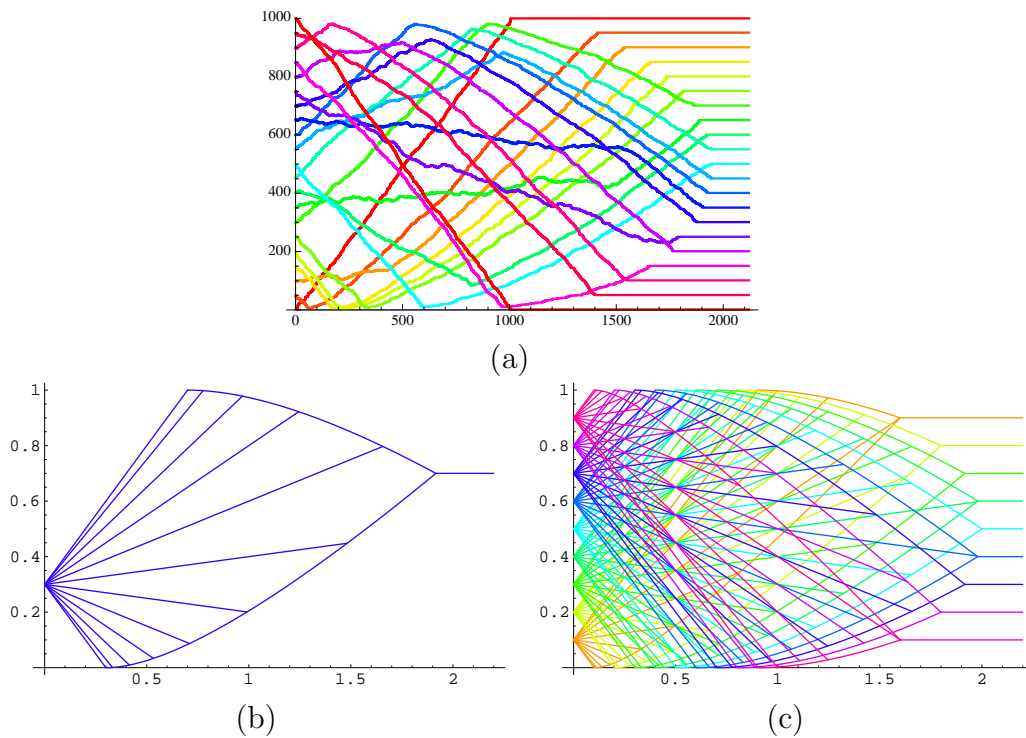
Figure 2: (a) Selected particle trajectories in a simulated oriented swap process with n = 1000 . (b) Selected possible limiting trajectories for particle \lfloor 3n/10 \rfloor . (c) Selected limiting trajectories (see Theorem 1.1).
