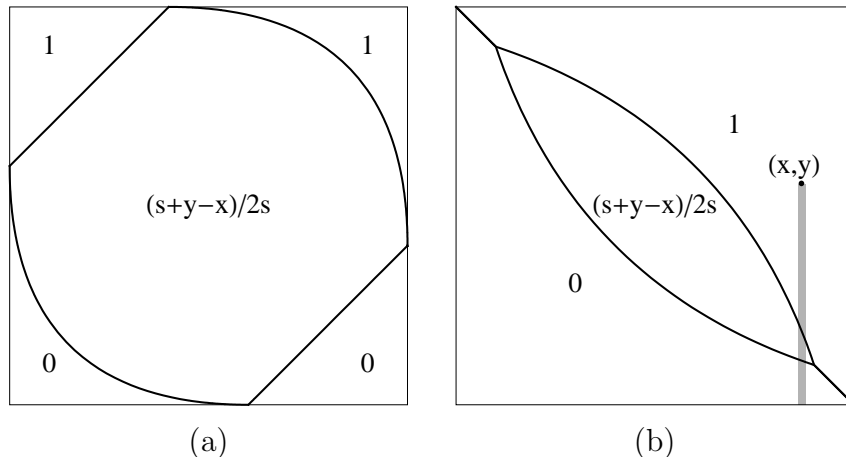
Figure 8: Values of g(s, x, y) in the (x, y) plane for (a) 0 < s < 1 and (b) 1 < s < 2 (there is no need to treat the boundary case s = 1 because of continuity in s ). To compute g(s, x, y) , integrate \kappa_s over the shaded thin strip of infinitesimal width.
