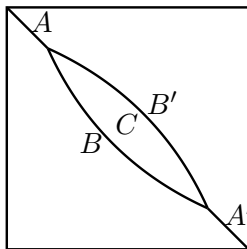
Figure 11: Contribution to I(s) for s > 1 . A, A' : diagonal segments; B, B' : arcs; C : lens-shaped region between the arcs.
