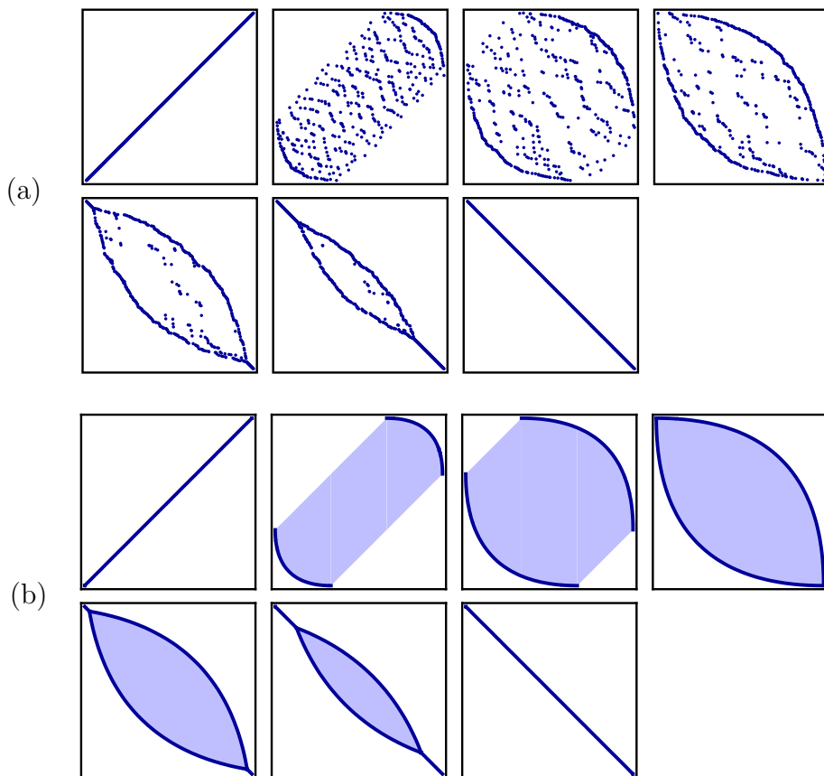
Figure 3: (a) The configuration (i.e. the support of the permutation matrix) at times 0, n/3, \dots, 6n/3 for a simulated oriented swap process with n = 500 . (b) An illustration of the limiting measures for these configurations as n \rightarrow \infty (see Theorem 1.2).
