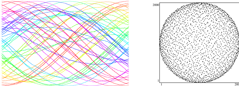
Figure 4: Selected trajectories and half-time configuration for a 2000-element uniform sorting network.
