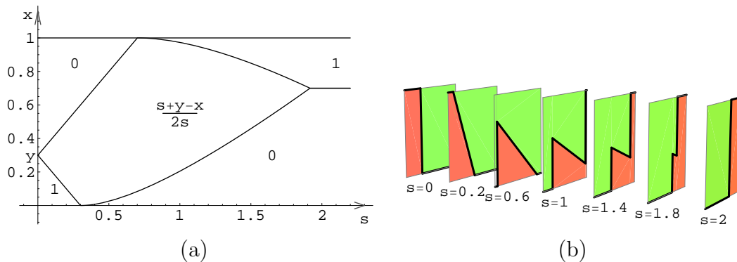
Figure 6: (a) Schematic representation of f(s, x, y) in the (s, x) -plane for y = 0.3 . (b) Several time slices of f(s, x, y) (shown as a function of x ) for y = 0.3 .
