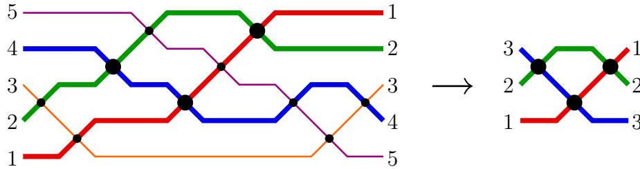
Figure 1: An illustration of the 5-particle sorting network \omega = (2, 1, 3, 4, 2, 3, 4, 2, 1, 2) , together with the 3-particle subnetwork \omega|_A = (2, 1, 2) induced by the subset of particles A = \{1, 2, 4\} .
