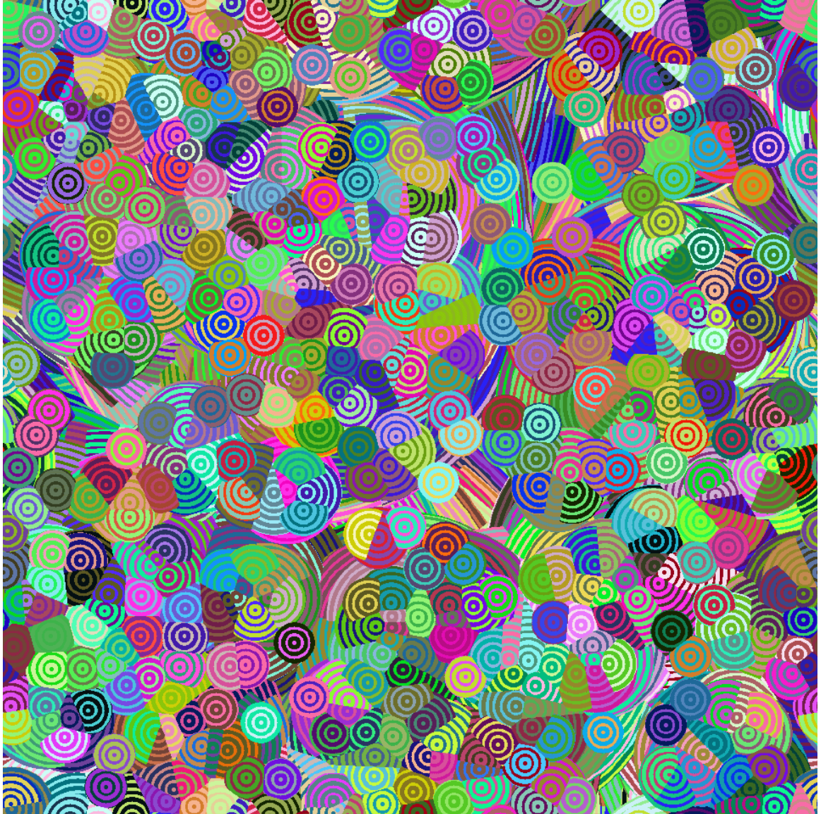
Figure 1: A stable allocation in the critical case \alpha = 1 . (If you are looking at greyscale images, color versions are available at http://www.math.ubc.ca/~holroyd or math.PR/0505668 ).
