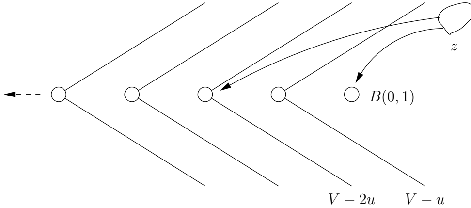
Figure 4: An illustration of the proof of Theorem 28(i). Some cone must contain an infinite volume of sites which desire all centers in the ball at its apex, and therefore it must also contain an infinite volume of sites which desire all centers in the ball B(0, 1) .
