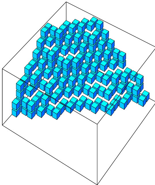
FIGURE 2. A good proto-brick with L = 4 . The set \widehat{S} comprises the (sites in the centers of) colored cubes. The origin is at the back corner, hidden by the set. The third coordinate axis is vertical.
