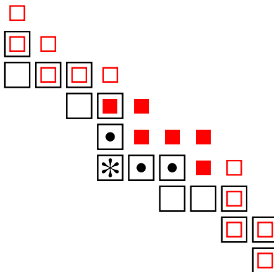
FIGURE 1. An illustration of the proof of Lemma 3. Two consecutive layers of a curtain are shown from above. Large squares are present in the upper layer, and small (red) squares in the lower layer. The argument showing that the upper layer site marked with a star becomes occupied is indicated. We consider the portion of the lower layer path shown by filled squares, and deduce that all the upper layer sites marked with discs become occupied.
