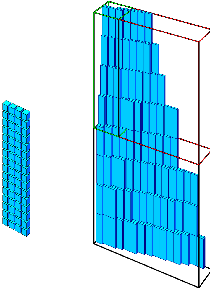
FIGURE 3. Left: An example of a cell \text{cell}(x) , which is a box of dimensions (1, 4, 16) . Right: A good brick B and its sail S for L = 4 . This is obtained by scaling the set \widehat{S} of Figure 2 and replacing each of its sites with a cell. The head of the brick is outlined in red, and its tip in green. Again, the distinguished corner, the origin, is at the back, hidden by the sail.
