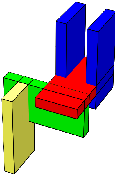
FIGURE 4. Illustration of the proof of Lemma 12. The initial brick B (at lower left) is yellow, and B_1 = B'_1 is green. The red box depicts B_2 and B'_2 , which are the same box but with different orientations. Finally, the two blue bricks are B_3 and B'_3 . These are translations of B by (10, 22, 22)L and (22, 22, 22)L .
