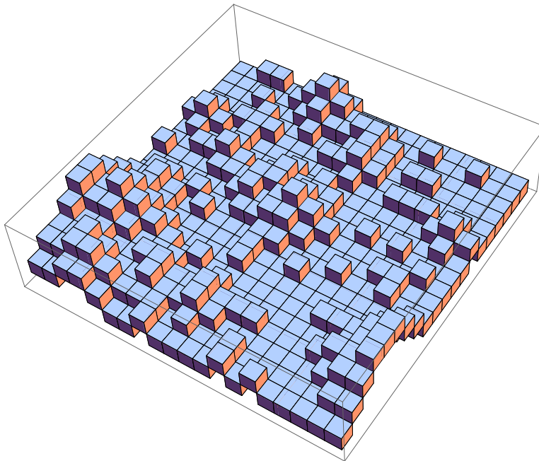
FIGURE 1. The lowest open Lipschitz surface (on a finite torus) when d = 3 and p = 0.82 . Each cube represents an open site in the surface.
