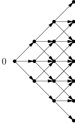
FIGURE 2. Part of the lattice \vec{\mathbb{L}}_{\text{alt}}^2 of [13], obtained by adding oriented edges to \mathbb{Z}^2 .
