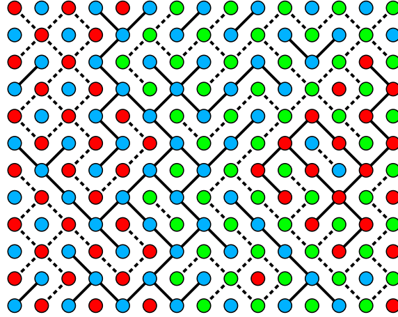
FIGURE 2. Random diagonals, the resulting bond percolation process (solid lines), its planar dual (dashed lines), and a corresponding 3-coloring.
